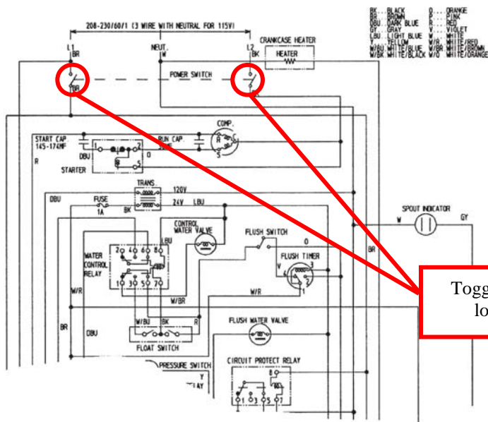
Original Wiring
