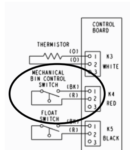
(New Mechanical bin control wiring)
