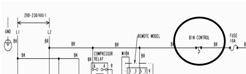
(Previous thermostatic bin control wiring)
