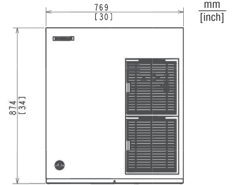
REMOTE AIR-COOLED
