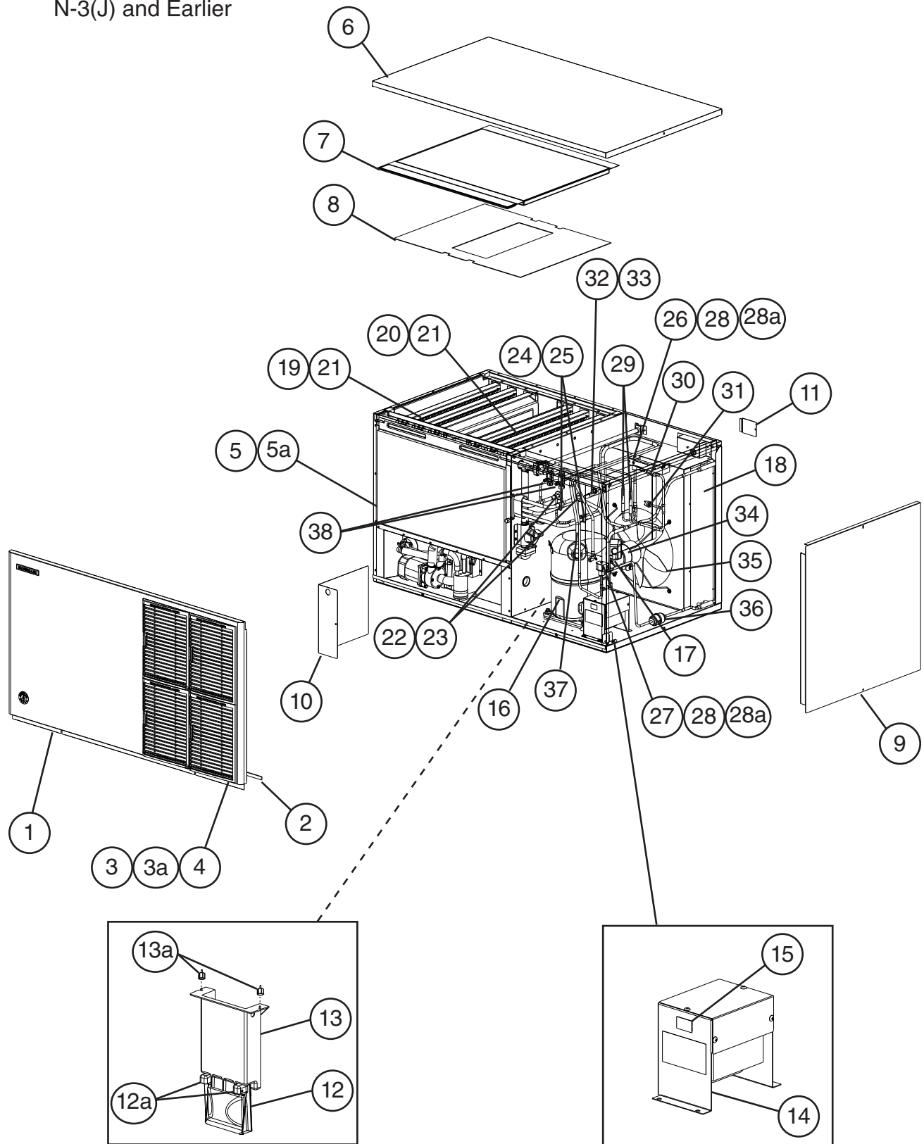
Main Transformer Box Assembly KM-1301SAJ3
